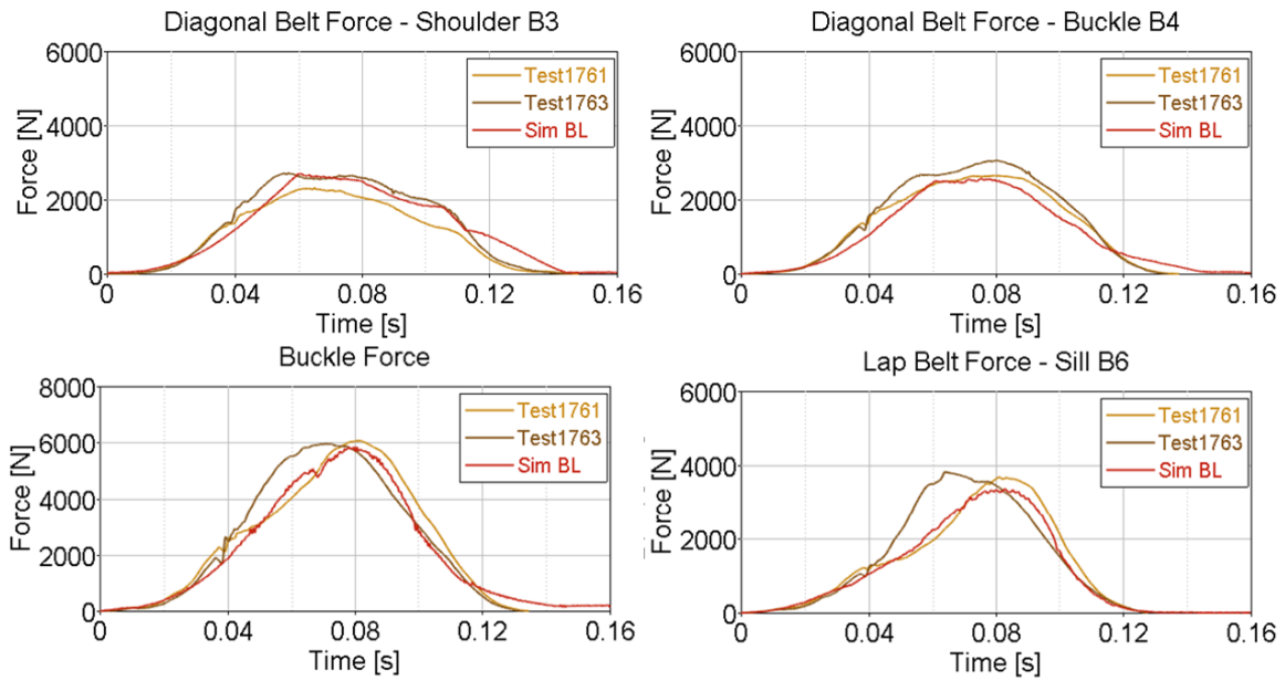
Figure A.3 Comparison of the time history of seat belt forces between PMHS 1 and PMHS 2 and the THUMS model in test conditions 1.
