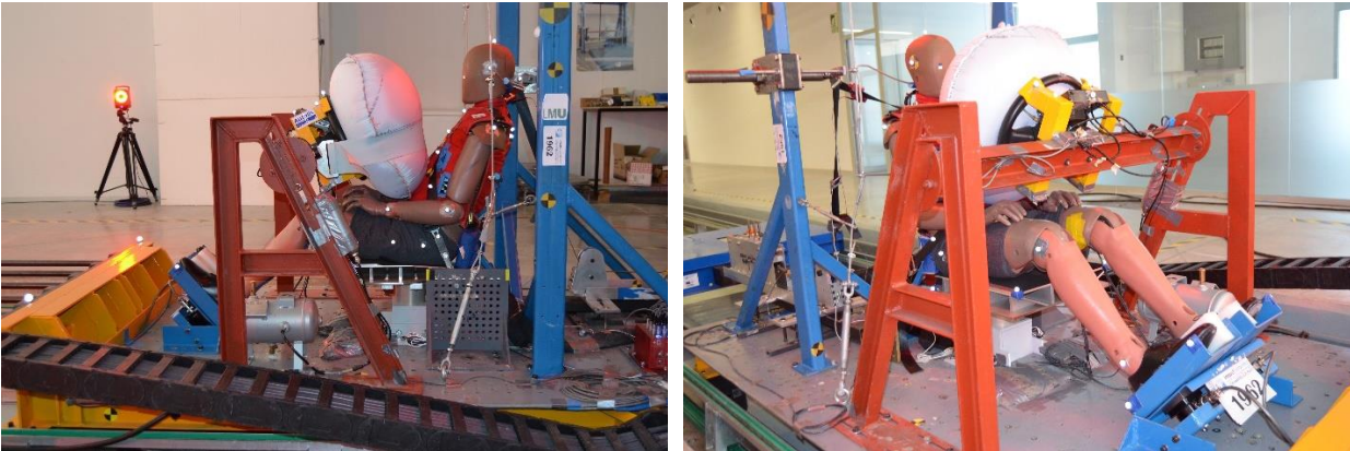
Figure A. 1 Generic oblique and lateral view of the test fixture and seating position of the THOR dummy (Cond. B). Notice the initial contact between the airbag and the dummy.
