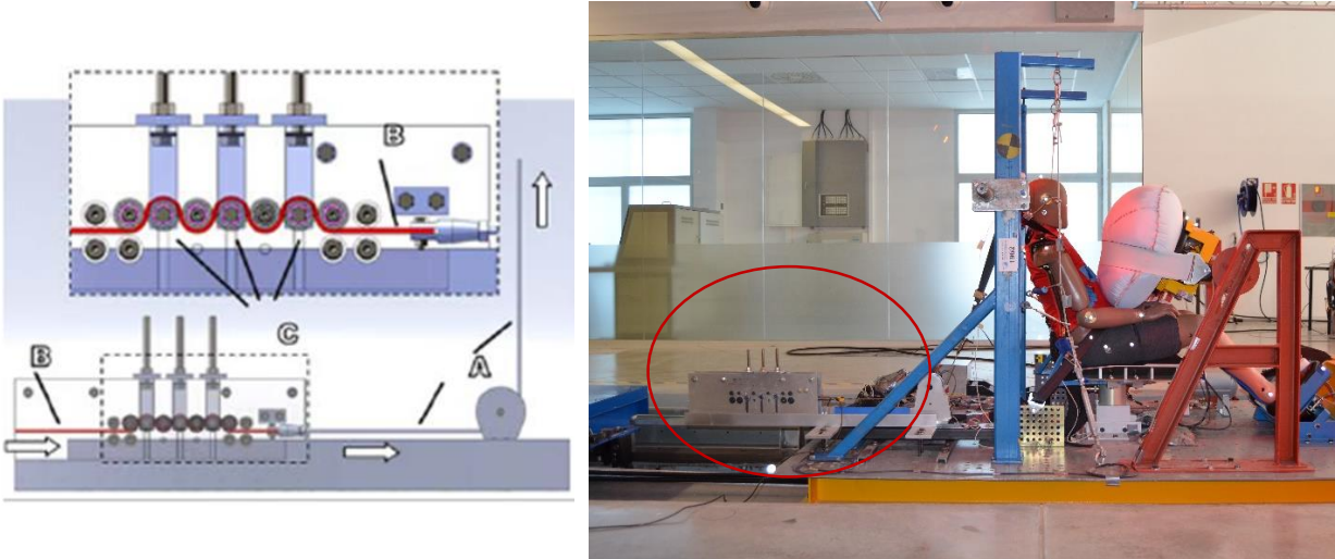
Figure A. 2 Illustration of the generic load limiting device and picture showing its position on the test fixture.
