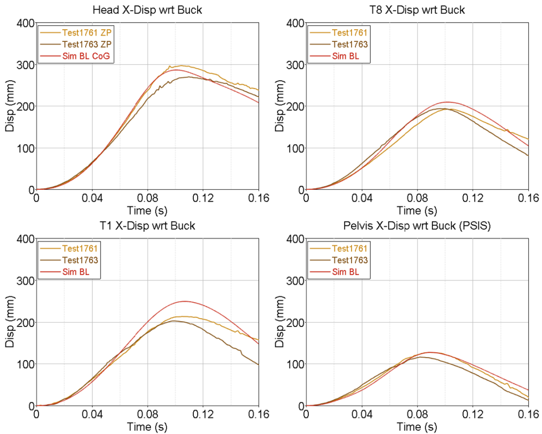
Figure A.4 Comparison of the time history of the X displacement of selected anatomical landmarks between PMHS 1 and PMHS 2 and the THUMS model in test conditions 1.
