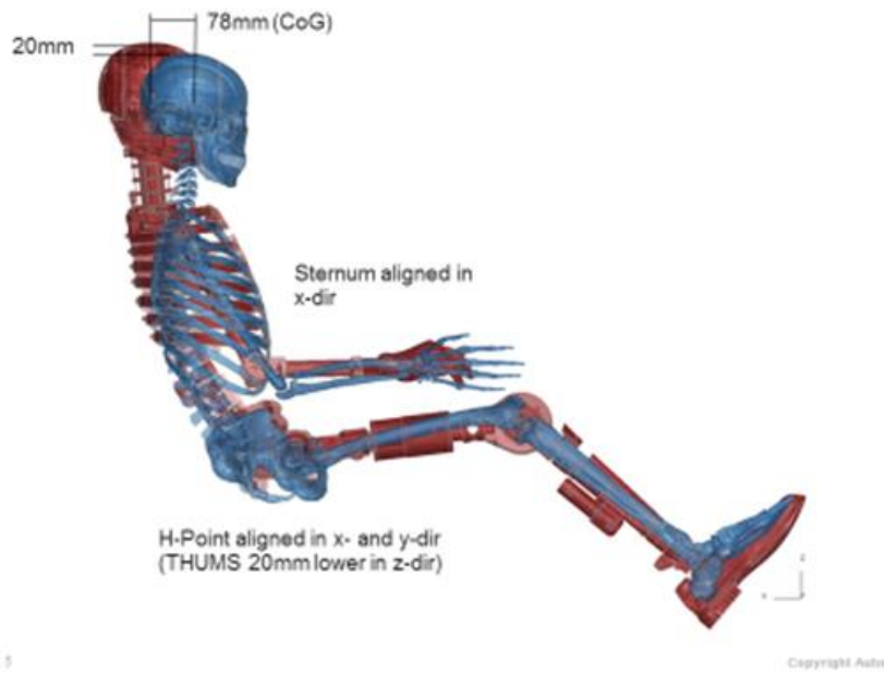
Figure A. 5 Comparison of the initial seating position between the THOR M dummy finite element model and the THUMS model
